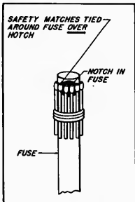
Time Fuse Fire Starter
